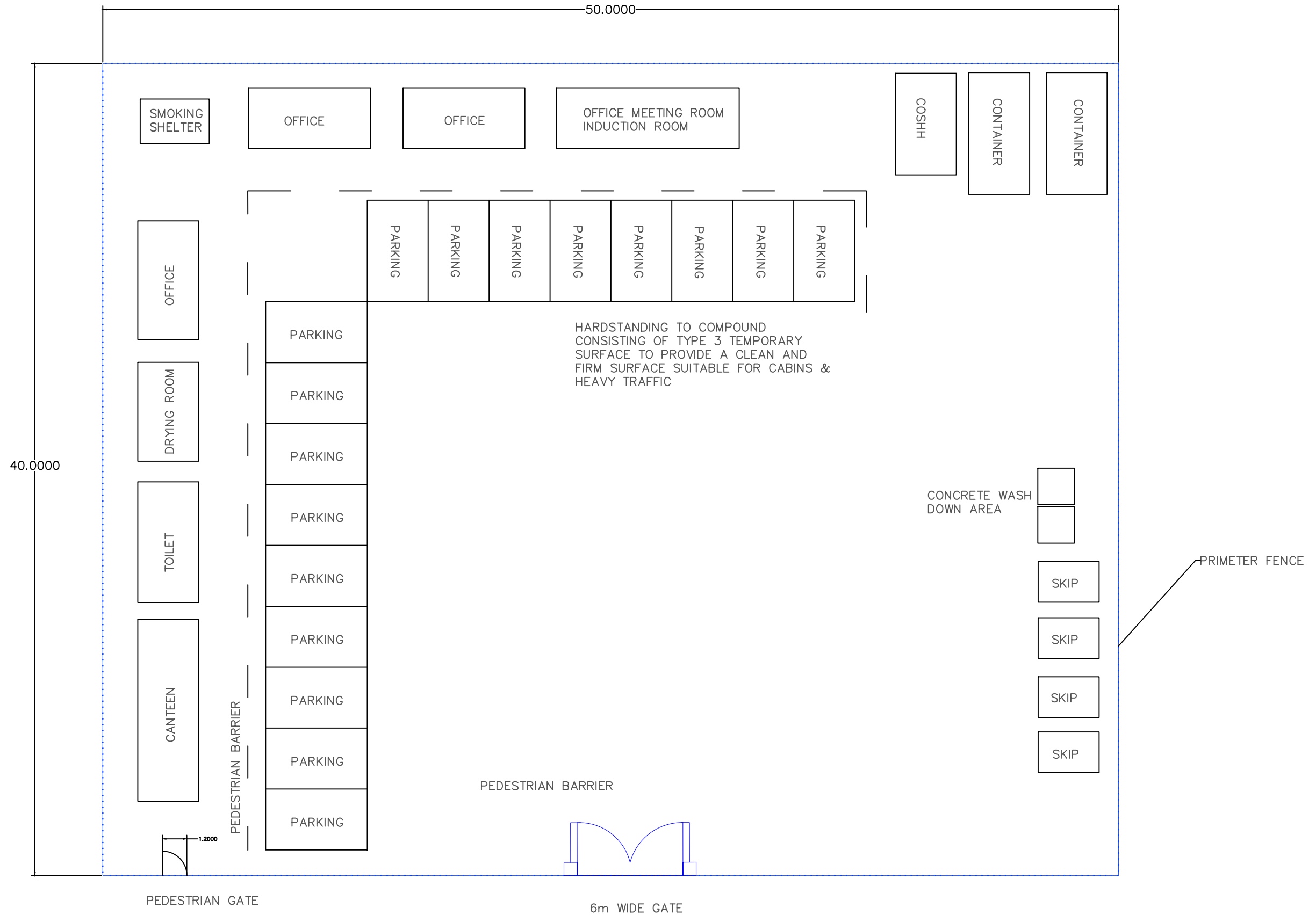
TEMPORARY CONSTRUCTION COMPOUND PLAN 1:200
